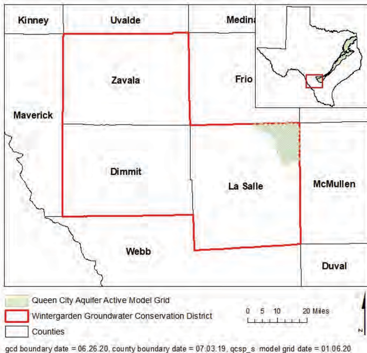
FIGURE 3: AREA OF THE GROUNDWATER AVAILABILITY MODEL FOR THE SOUTHERN PORTION OF THE CARRIZO-WILCOX, QUEEN CITY, AND SPARTA AQUIFERS FROM WHICH THE INFORMATION IN TABLE 3 WAS EXTRACTED (THE QUEEN CITY AQUIFER EXTENT WITHIN THE DISTRICT BOUNDARY).
